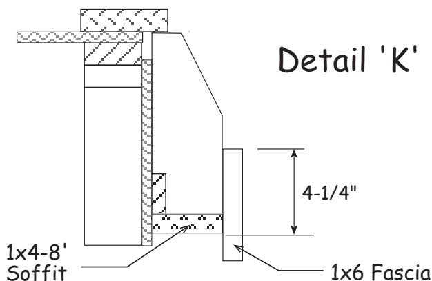
1x4-8' Soffit Board
