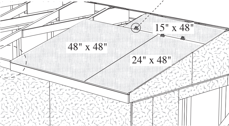
Roof Ridge
