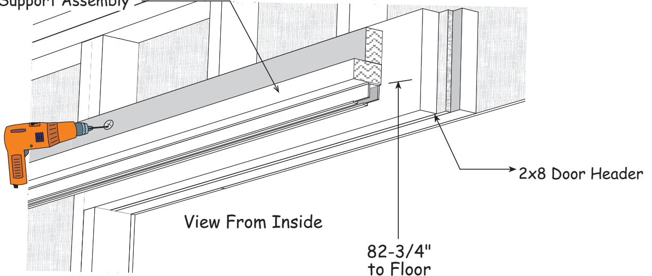
2x3 Track Support Assembly
